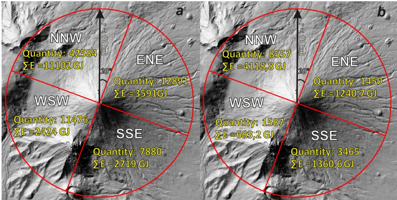
Fig. 1. The region of the Klyuchevskoi Volcano with a radius of 10 km is divided on into sectors with calculations of total quantity of earthquakes and their energy for data for 1995-2017: a - for all range of data ( h \leq 5 \div - 50 km); b - for earthquakes in construction (with h \leq 5 \div 0 km).
